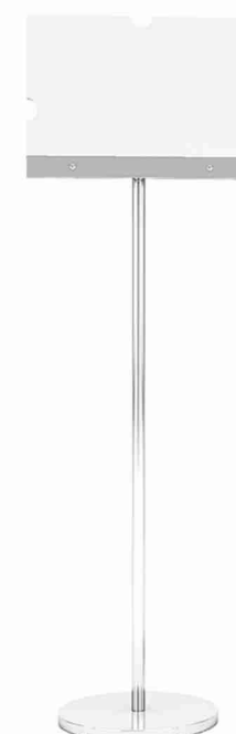
1842 SIGN BOARD » AISI 304 Stainless steel pipe body and the base » Plexiglass frame (A4) Dimensions Ø:30 H:120 cm
